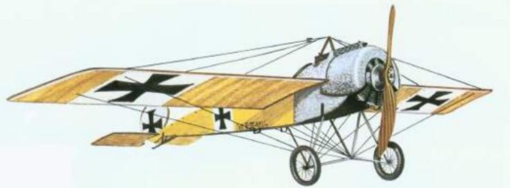
Oswald Boelcke and his Fokker E.III, built 1915, powered by Oberursel U.I 9-cylinder air-cooled rotary 100 HP engine, weighed 1,342 lbs., max. speed of 88 MPH, max. ceiling of 11,500 feet, 1 synchronized Spandau machine gun
